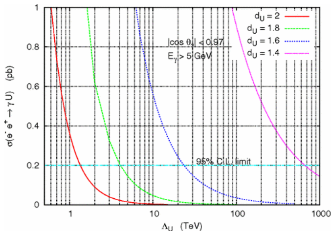
Figure 2: Cross sections for mono-photon plus unparticle production at the e^+e^- collider with \sqrt{s} = 207 GeV for d_U = 1.4, 1.6, 1.8 and 2 . The horizontal line of 0.2 pb is the 95% C.L. upper limit, from [4].
