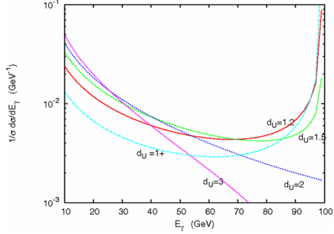
Figure 1: Mono-photon energy spectrum for the process e^+e^- \rightarrow \gamma\mathcal{U} for d_{\mathcal{U}} = 1 + \epsilon, 1.2, 1.5, 2 and 3 at \sqrt{s} = 200\text{GeV} . We have imposed |\cos\theta_\gamma| < 0.95 , from [6].
