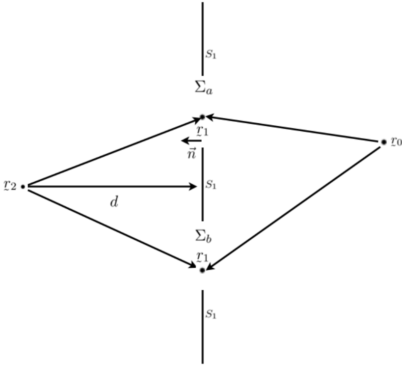
Figure 7: Two circular slits, \Sigma_a and \Sigma_b , with point source at \mathcal{L}_2 which is at distance d from the slit and situated midway of the two slits; the wave function in the ambient environment on the left of the slit is diffracted on the right of the slit
