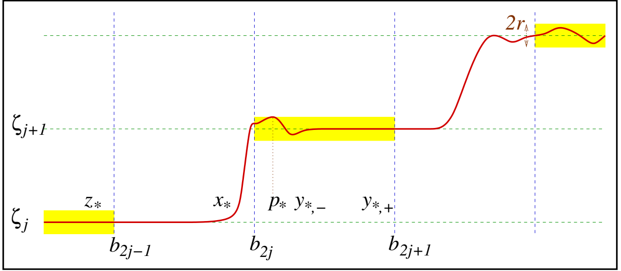
FIGURE 4. The points z_* , x_* , p_* , y_{*,-} and y_{*,+} .
