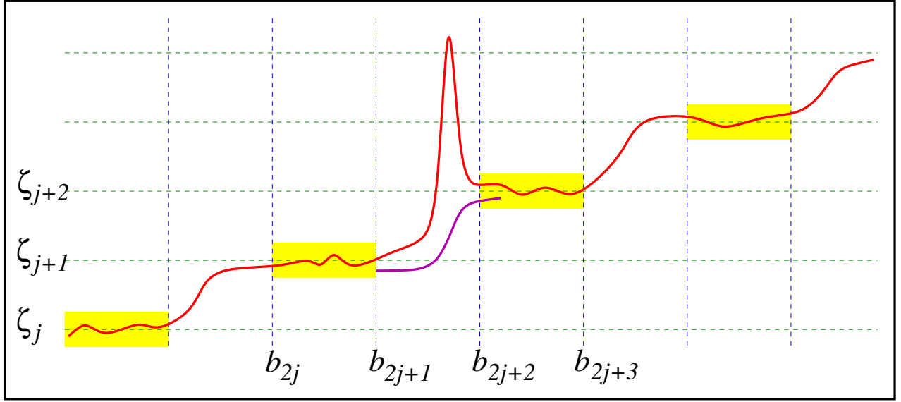
FIGURE 3. Glueing Q_* with Q_*^{\zeta_{j+1}, \zeta_{j+2}} .
