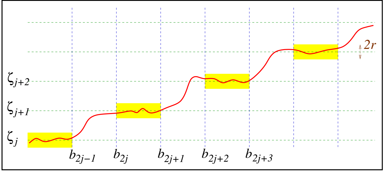
FIGURE 2. The sets of admissible competitors in \Gamma(\vec{\zeta}, \vec{b}) .
