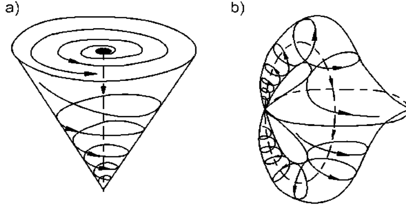
Figure 1: \omega(x, k) -, but not \Omega(x, k) -bifurcations: a - phase portrait of the system (14); b - the same portrait after gluing all fixed points.
