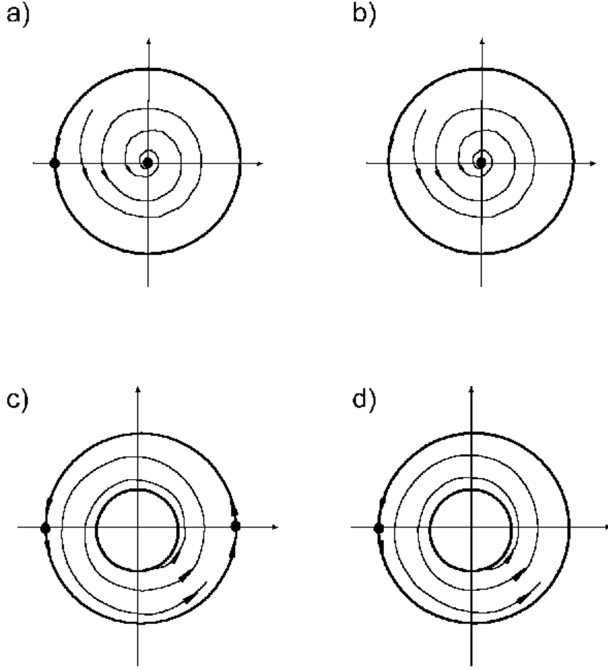
Figure 2: Phase portraits of the systems: a - (15); b - (16); c - (17); d - (18)
