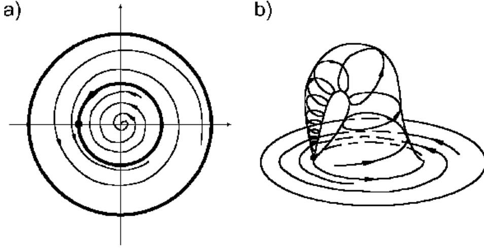
Figure 3: Phase portrait of the system (19): a - without gluing the fixed points; b - after gluing.
