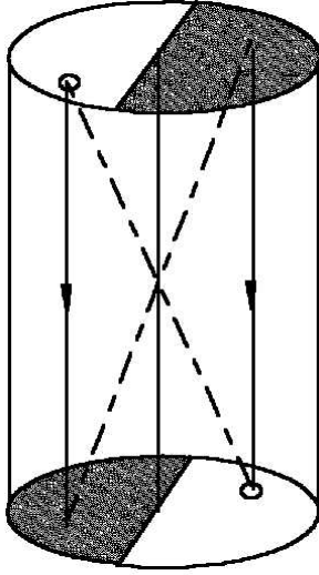
Figure 5: Phase space of the system (Example 3.1). All the points of the axis are non-wandering; \circ is the place of delay near fixed points.
