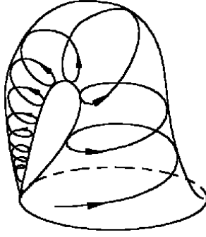
Figure 4: Phase portrait of the system (15) after gluing the fixed points.
